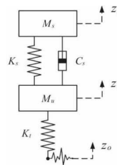
Fig. 2. A theoretical model of passive suspension [14]
