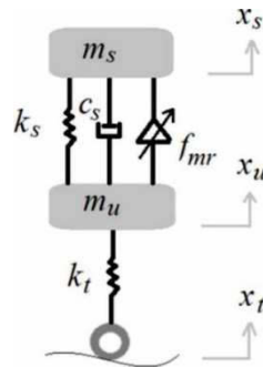
Fig. 3. A theoretical model of a semi-active suspension system [16]
