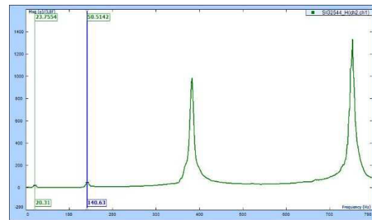
Fig. 3. Modal frequencies of an inclined cracked composite beam
