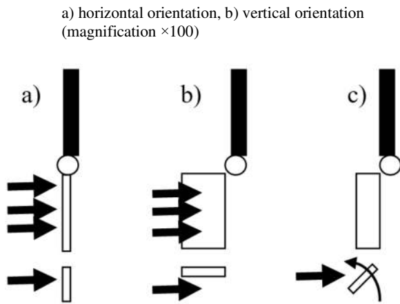
Fig. 8. Types of workpiece surface orientation in a vertical arrangement
