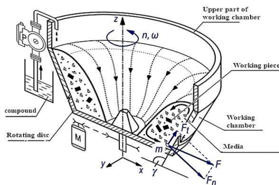
Fig. 1. The paths of movement of the abrasive media in the working container of the disc centrifugal machine [1, 2]
