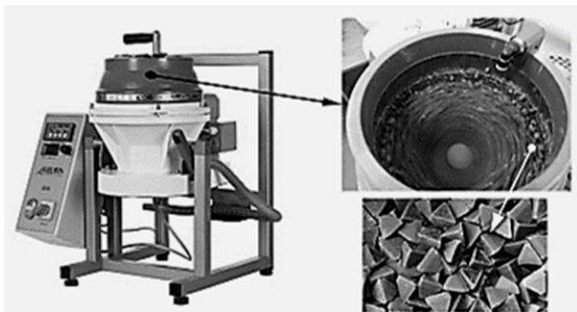
Fig. 3. EC6 rotary container smoothing machine
