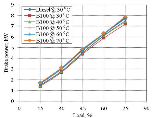
Fig. 3. Output engine power at different loads
