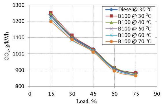
Fig. 7. CO 2 emission of engine at different loads
