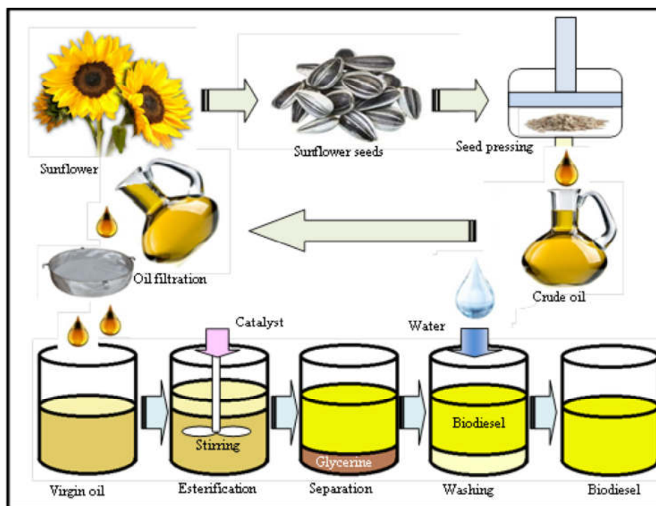
Fig. 1. Schematic diagram of biodiesel production procedures
