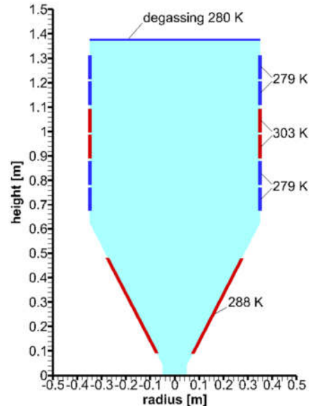
Fig. 7 Boundary conditions in the second case
