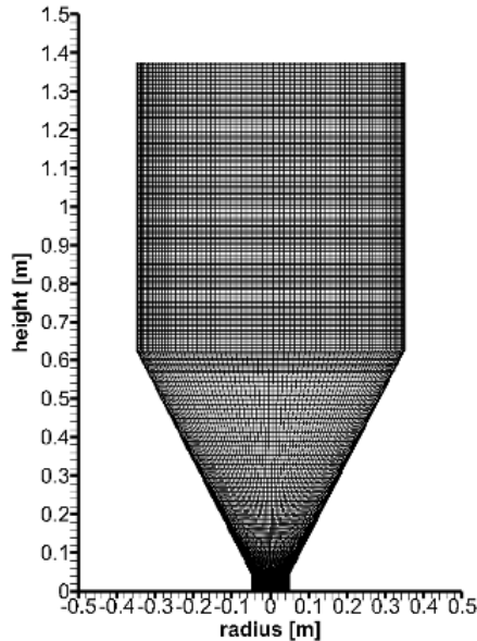
Fig. 5 Meshing of the fermentation tank (front view)
