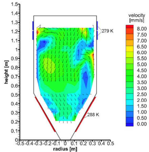
Fig. 12 Velocity field and vector plot in the cylindrical tank with conical bottom after 1 hour, UDV, first case
