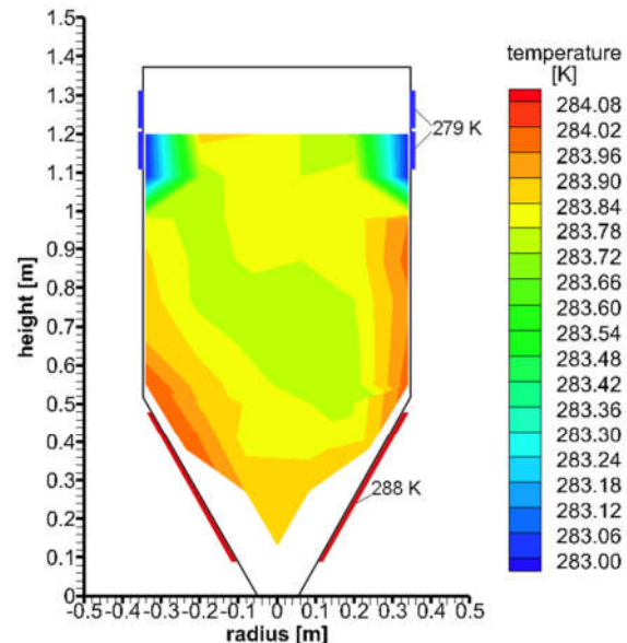
Fig. 8 Temperature field inside the cylindrical tank with conical bottom in the first case, experimental result after 1 hour
