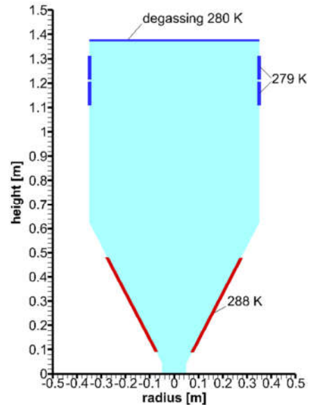
Fig. 6 Boundary conditions in the first case
