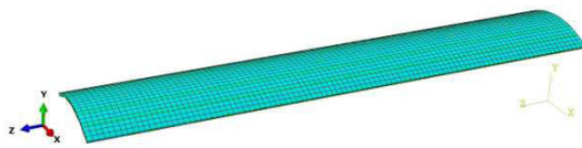
Fig. 3. Free meshing technique with linear tetrahedral and hexahedral elements
