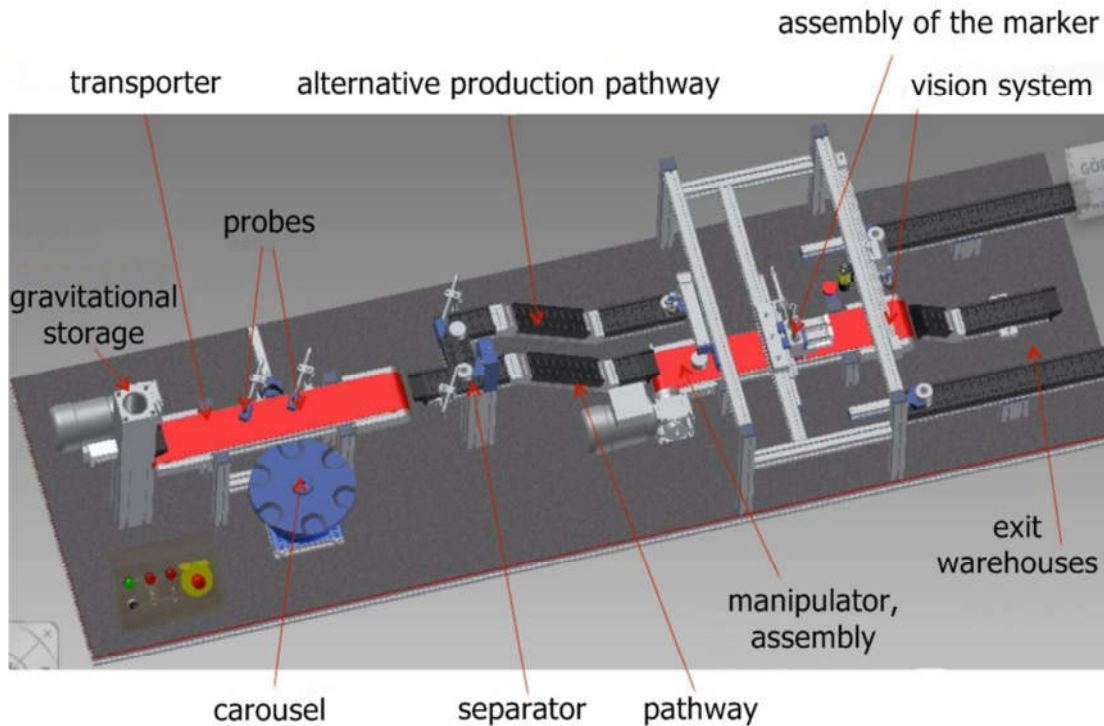
Fig. 2. View of the teaching station [3]
