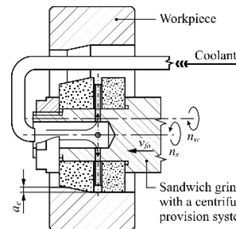
Fig. 9. Cross-section of the grinding zone using sandwich grinding wheel [10]
