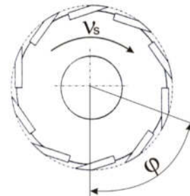
Fig. 5. Grinding fluid outflow angle \varphi in method using T-Tool-Profil grinding wheel [21]
