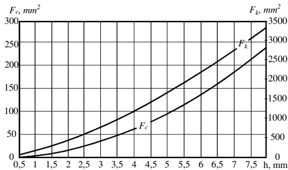
Fig. 3. Comparison of calculated values of area of slice section F_c and contact area F_k of grinding wheel.
