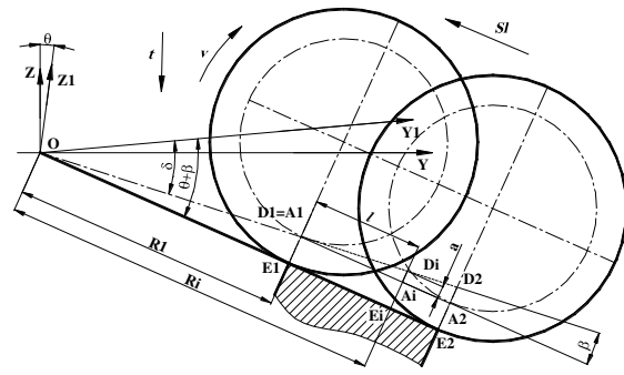
Fig. 1. The deep profiled grinding of gear
