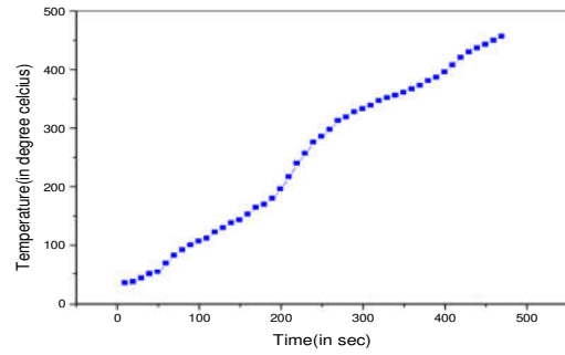
Fig. 2. Heating curve of AISI1040 steel
