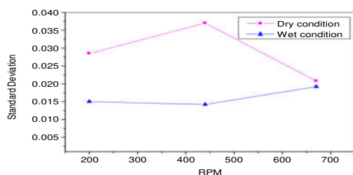
Fig. 6. Standard deviation vs. rpm curve (8 mm)
