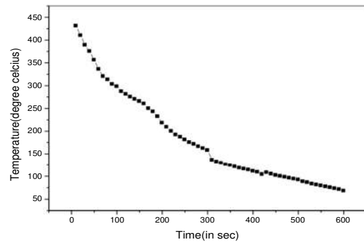
Fig. 3. Cooling curve of AISI1040 steel (air cooling)
