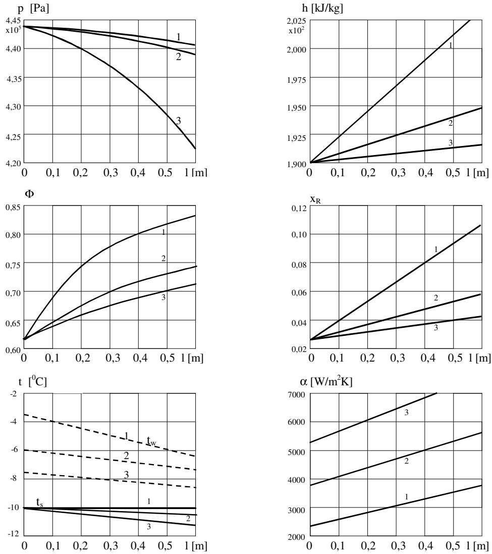
Fig. 7. The distribution of quantities describing the process of bubble boiling of refrigerant RR404A as a function of axial coordinate of the horizontal channel: q = 15\,000\text{ W/m}^2 , T_{oi} = -10\text{ }^\circ\text{C} , p_i = 0,444\text{ MPa} , h_i = 190\text{ kJ/kg} , w\rho_i = 200\text{ kg/m}^2\text{s} , w\rho_2 = 600\text{ kg/m}^2\text{s} , w\rho_3 = 1600\text{ kg/m}^2\text{s}
