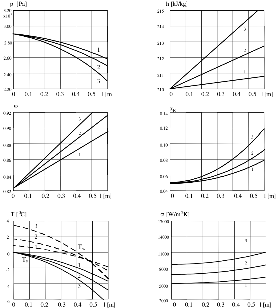
Fig. 6. The distribution of quantities describing the process of bubble boiling of refrigerant R134a as a function of axial coordinate of the horizontal channel: T_s = 0^{\circ}\text{C} , p_1 = 0.293 MPa, h_1 = 210 kJ/kg, (w_p) = 1000 kg/m 2 s, 1 - q_1 = 5000 W/m 2 , 2 - q_2 = 15000 W/m 2 , 3 - q_3 = 30000 W/m 2
