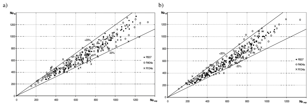
Fig. 8. The comparison of Nusselt number calculated from the presented model Nu_{th} and determined from own experimental investigations Nu_{exp} : a) horizontal channel, b) vertical channel
